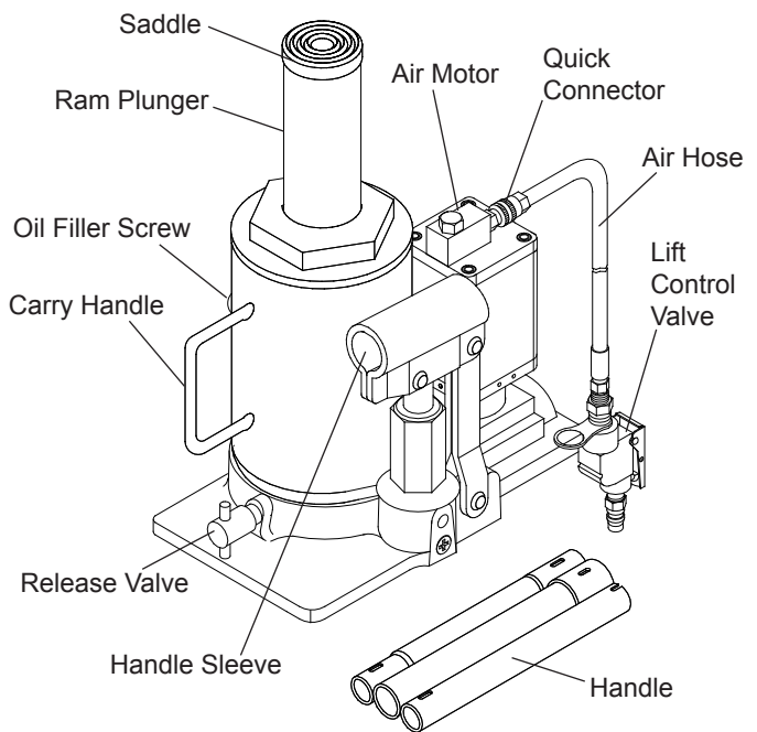
Figure 2 - 18302C Nomenclature
