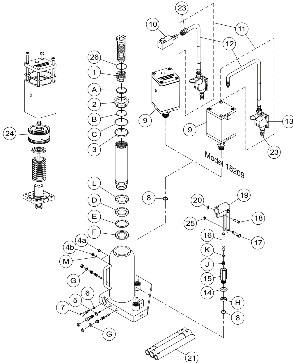
Figure 3 - Model 18122C, 18202C & 18209 Replacement Parts Illustration
