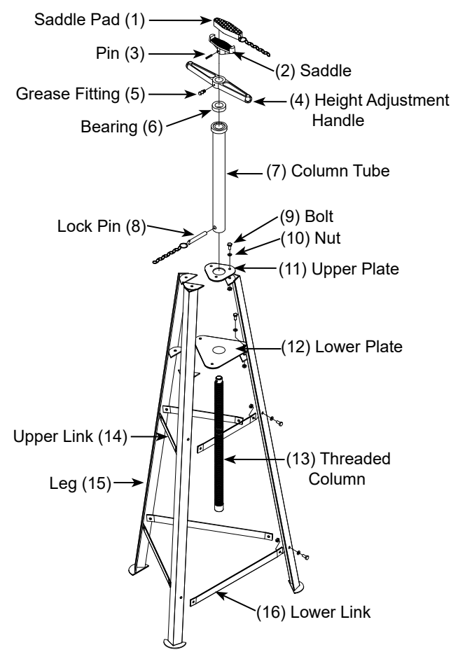
Figure 1 - Model 33020 Components
