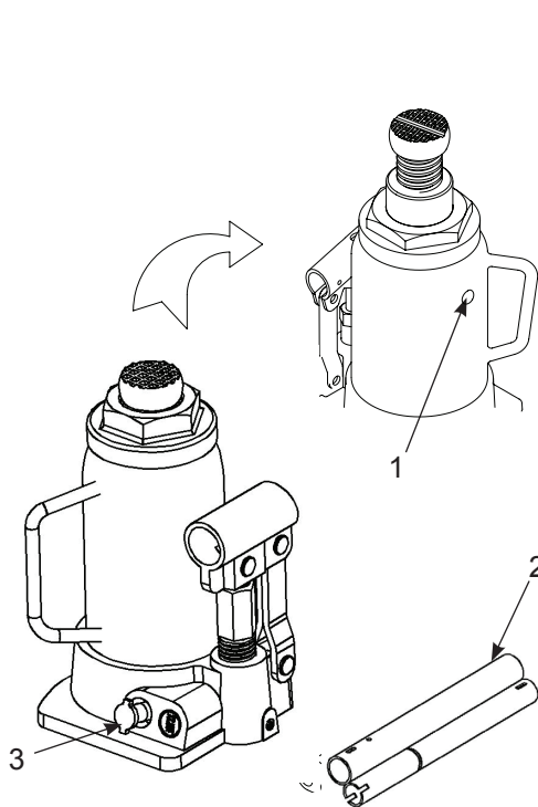
Figure 3 - Illustration for Models BH2080B, BH2120B & BH2020B
