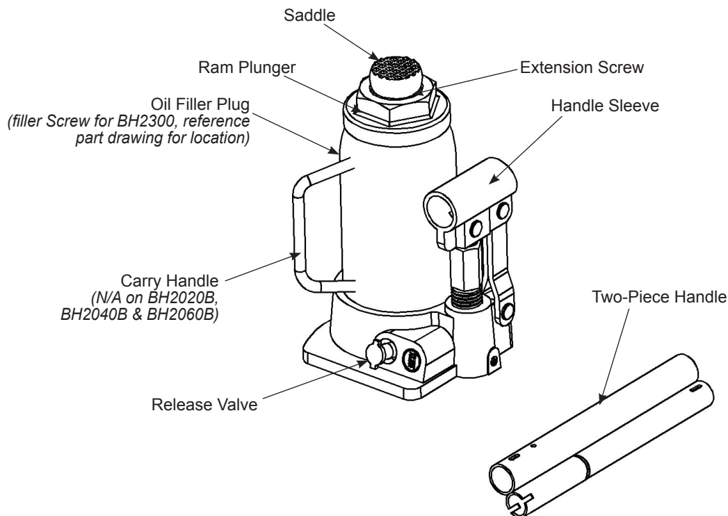
Figure 1 - Typical Bottle Jack Nomenclature (BH2200B shown)
