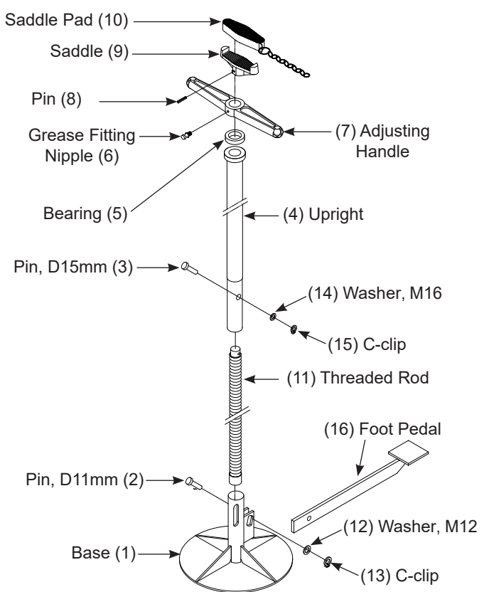
Figure 2 - BH5715 Nomenclature
