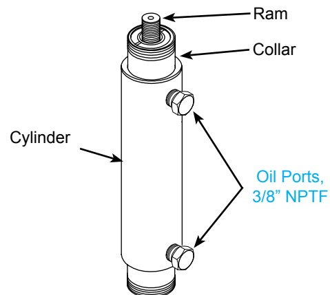
Figure 1 - Typical Cylinder Components
