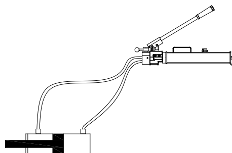
Figure 2 - Illustration to bleed air from system
