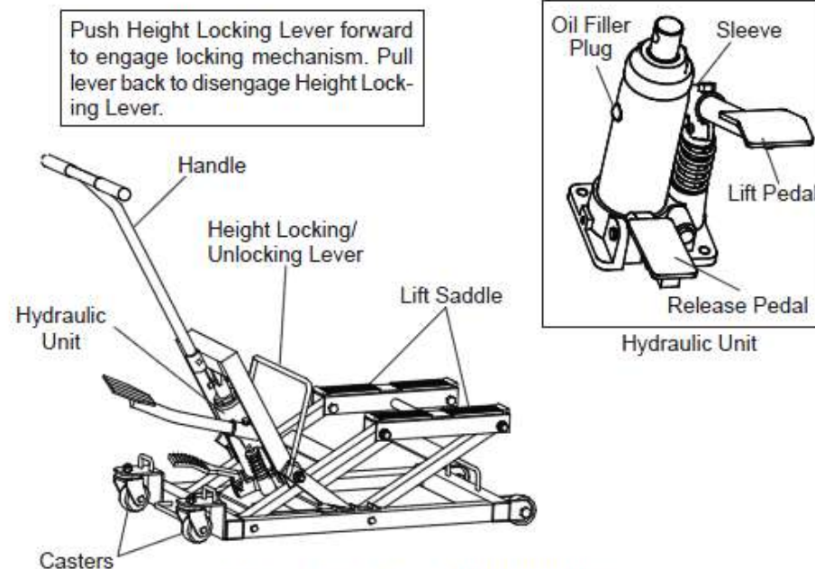
Figure 1 - Motorcycle/ATV Lift Nomenclature
