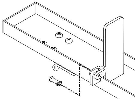
Figure 2 - Assembly of Stopping Plate to Wheel Track
