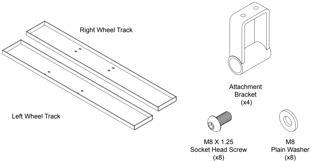
Figure 1 - Push Mower Adapter Nomenclature
